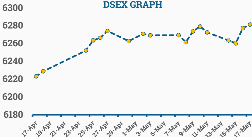
DSEX GRAPH
